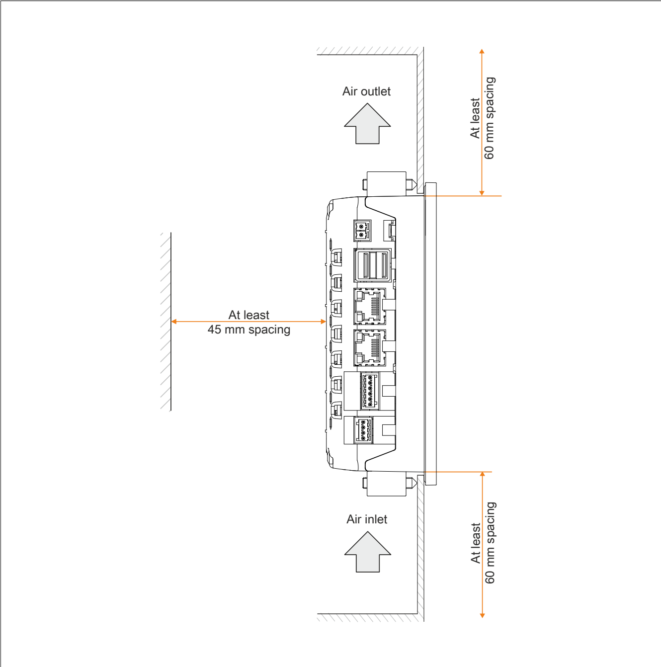
Figure 23: Spacing for air circulation - Side view
