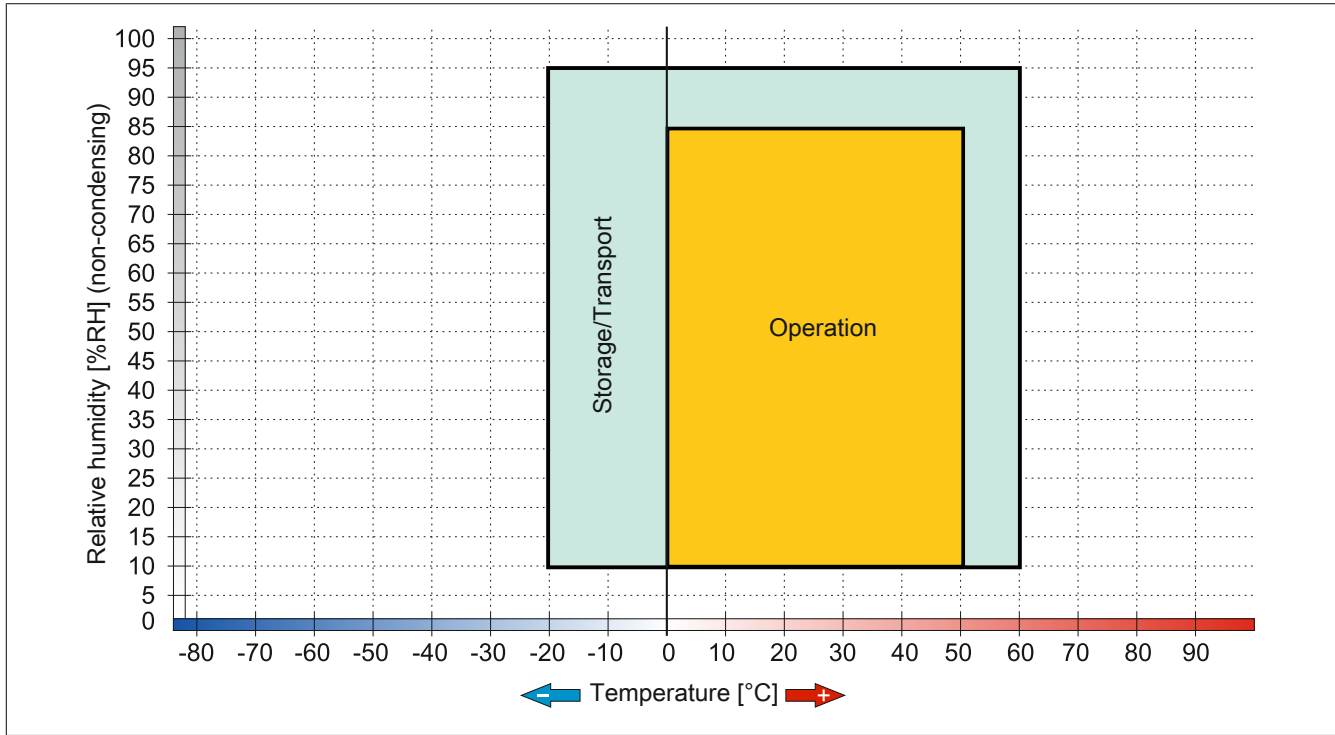
Figure 9: 4PPC70.101x-2xx - Temperature/Humidity diagram
