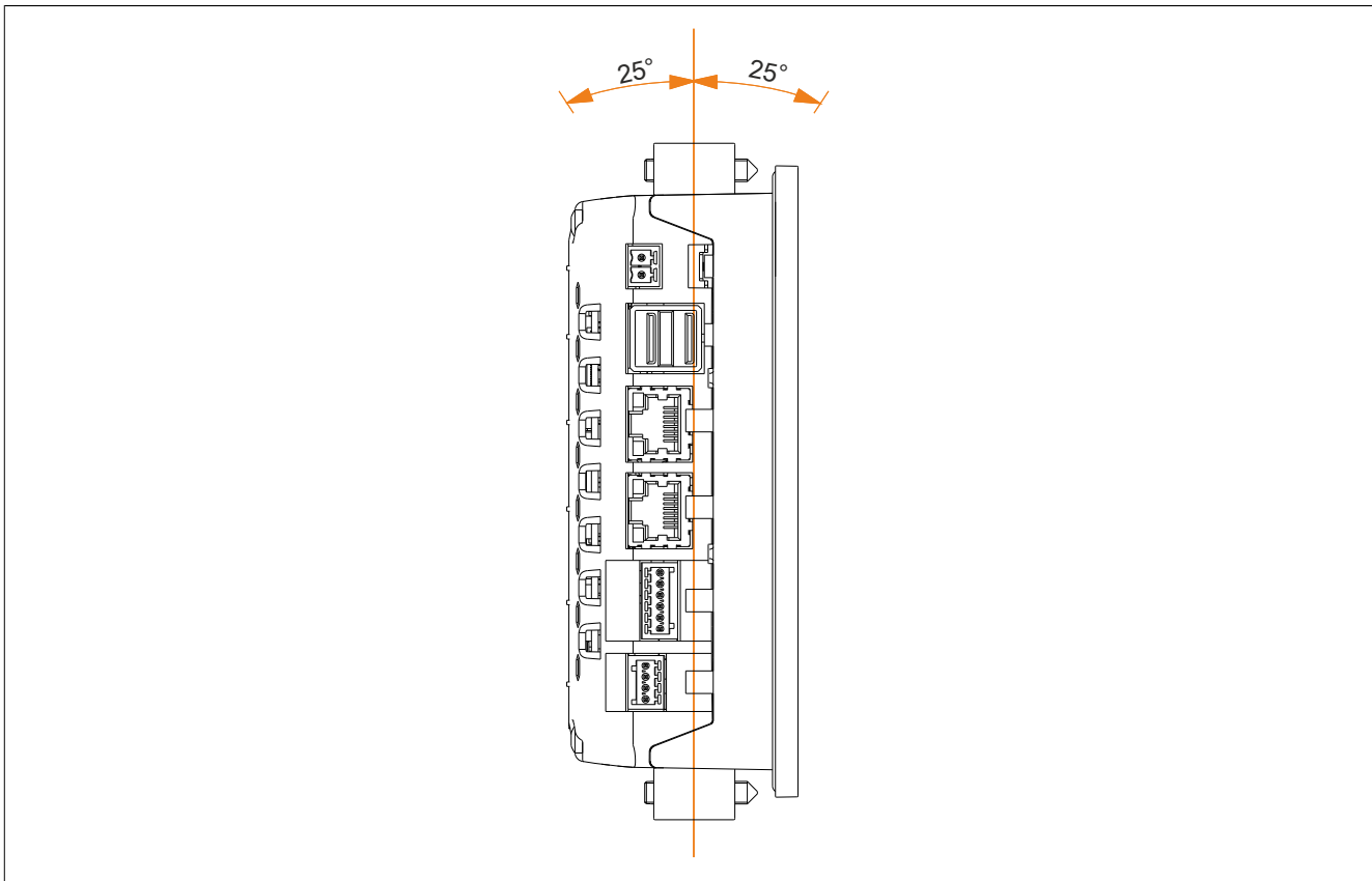
Figure 24: Power Panel - Mounting orientations
