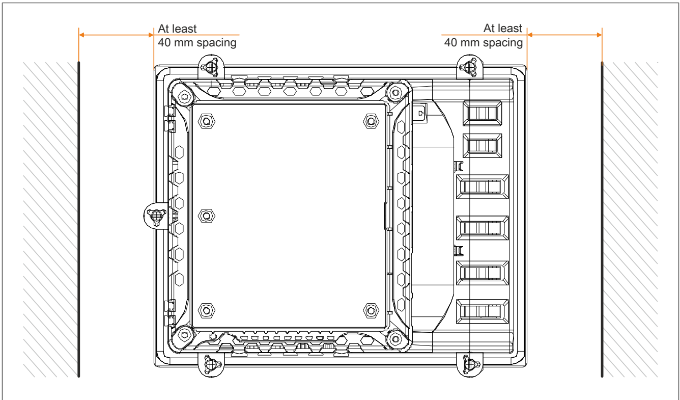
Figure 22: Spacing for air circulation - Rear view
