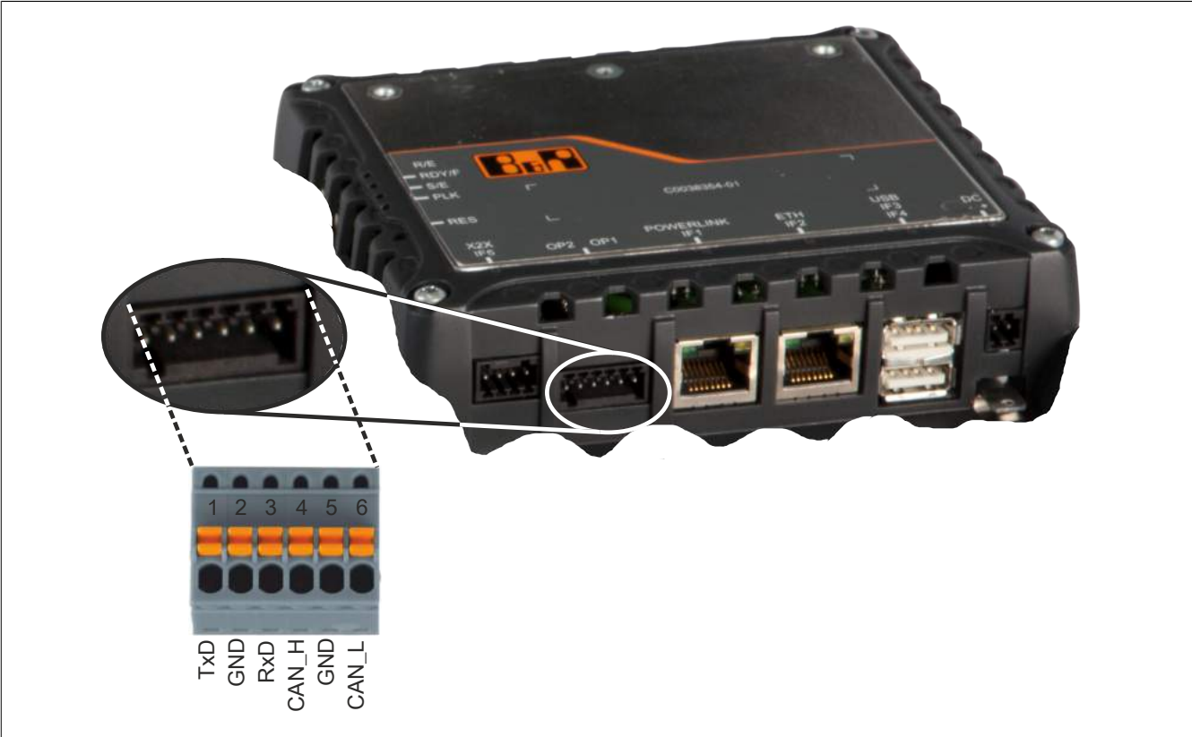
Figure 13: 4PPC70.xxxx-22x - 1 CAN bus interface / 1 RS232 interface
